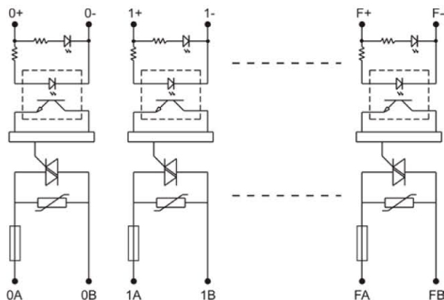
Schematic
